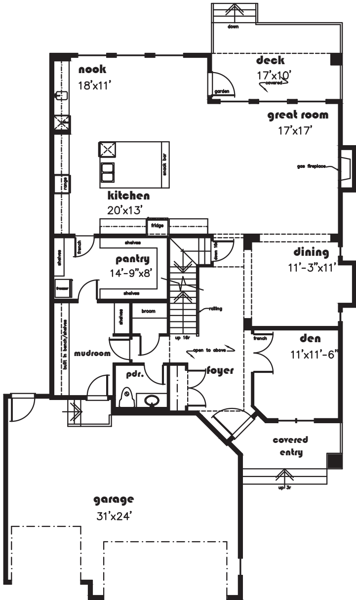
main floor 1705
