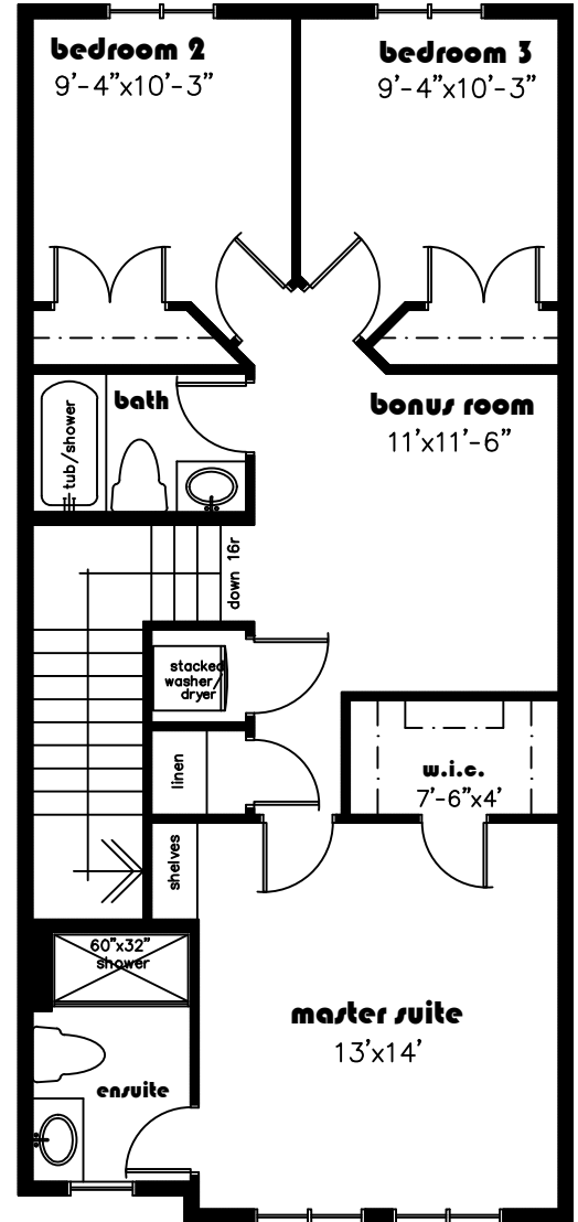
Second floor 800
