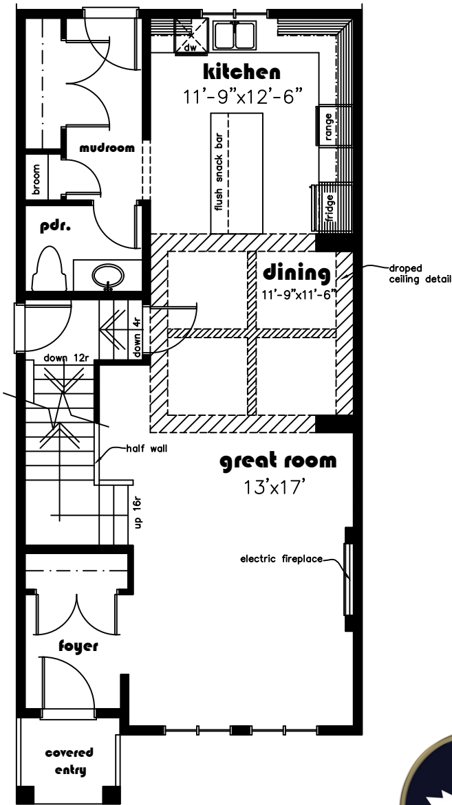
Main floor 834
