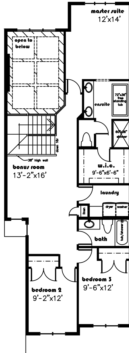
second floor 1093
